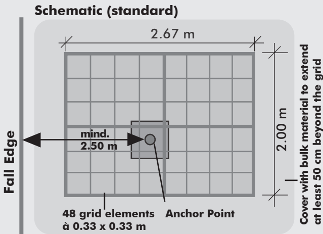
Schematic of a standard installation of the centred Anchor Point with the four pre-assembled grids (à 1.00 × 1.33 m).
