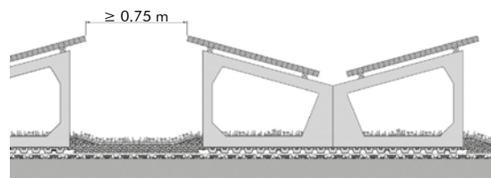
Solar Substructure Type "Butterfly"
