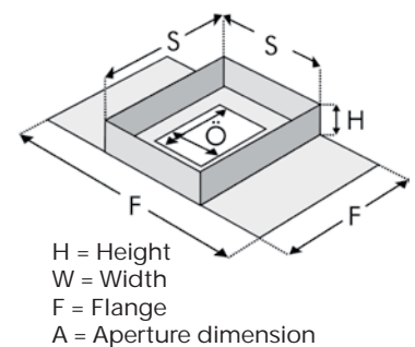
Inspection Chamber KS 6/30-GR and KS 10/30-GR with detachable galvanized grill
